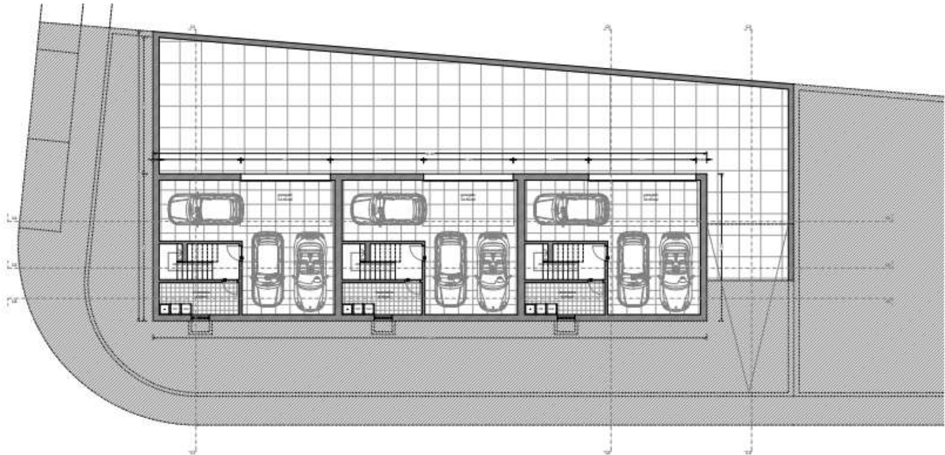
Cave 3 Moradias
