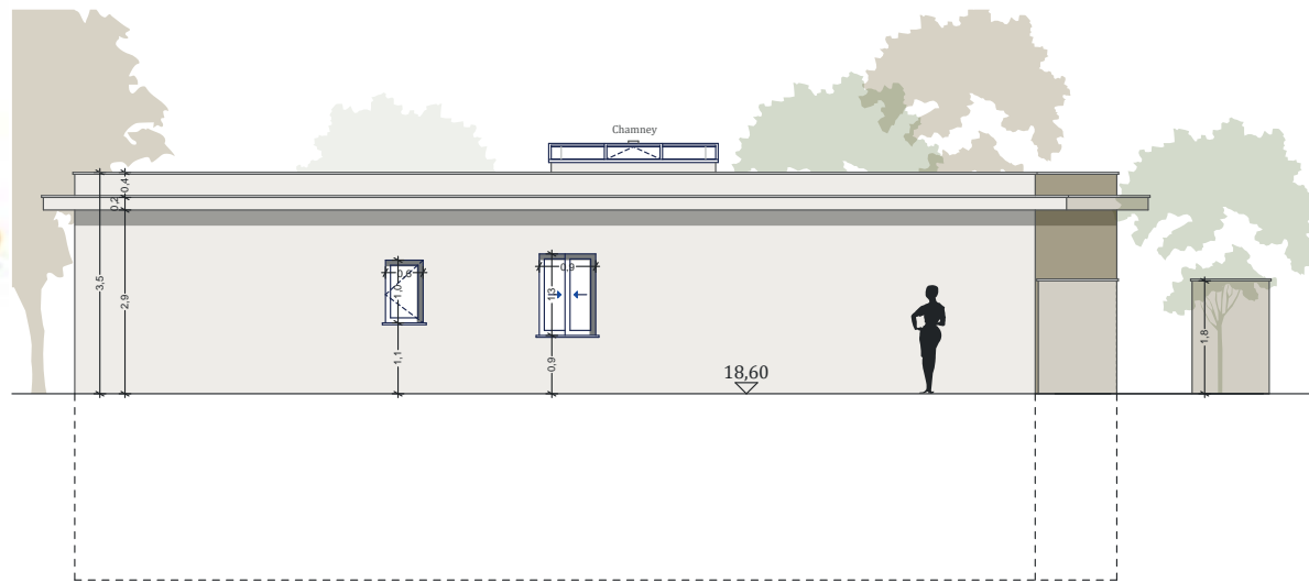
North elevation
