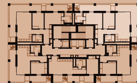
PLANTA PISO 11 | FLOOR PLAN 11
