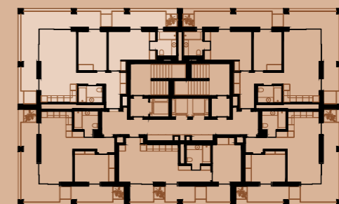
PLANTA PISO 20 | FLOOR PLAN 20
