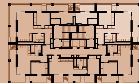
PLANTA PISO 17 | FLOOR PLAN 17
