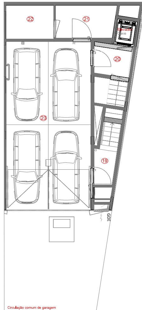
PISO CAVE
