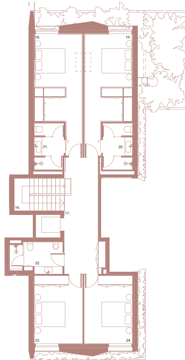
PISO 2 2ND FLOOR
