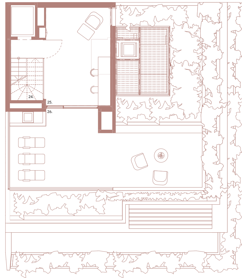
PISO 4 4TH FLOOR
