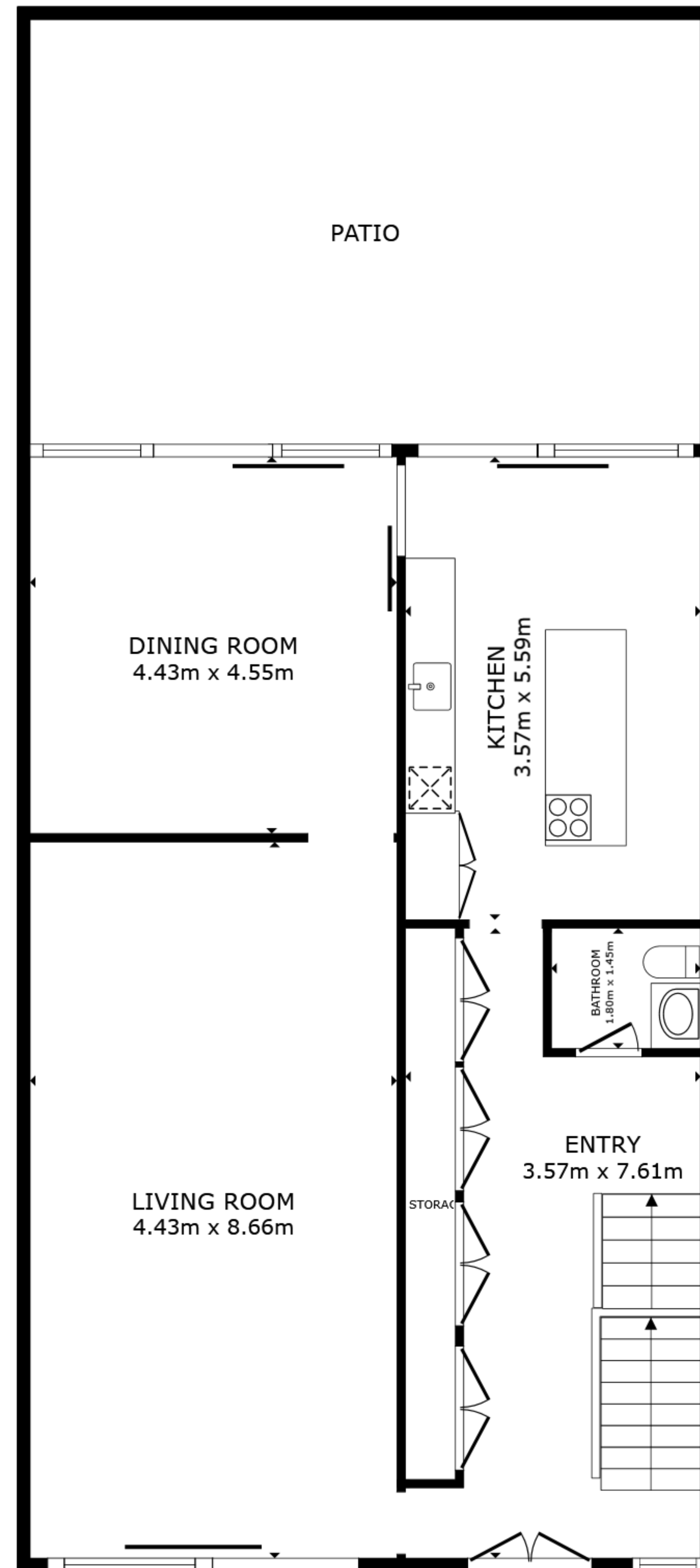
FLOOR 1
