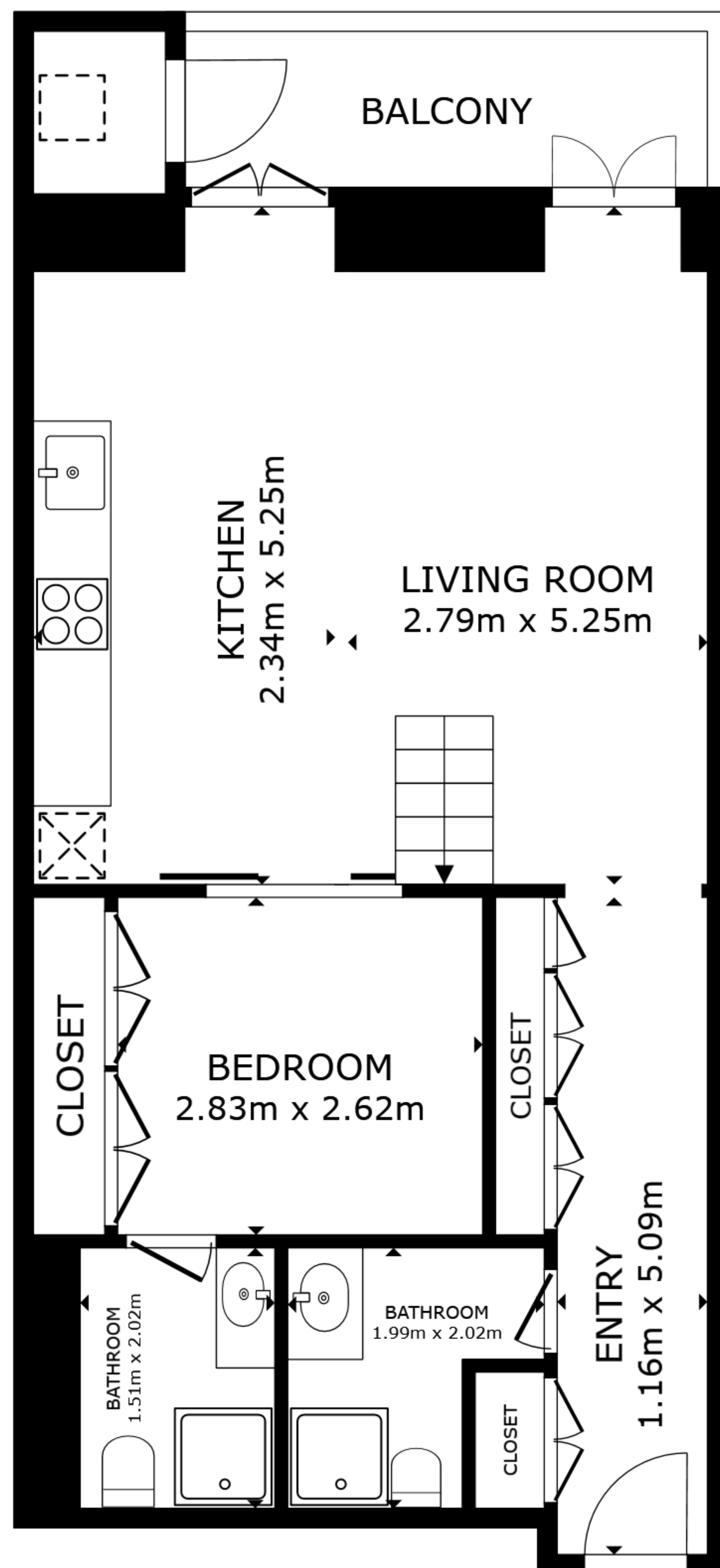
FLOOR 1
