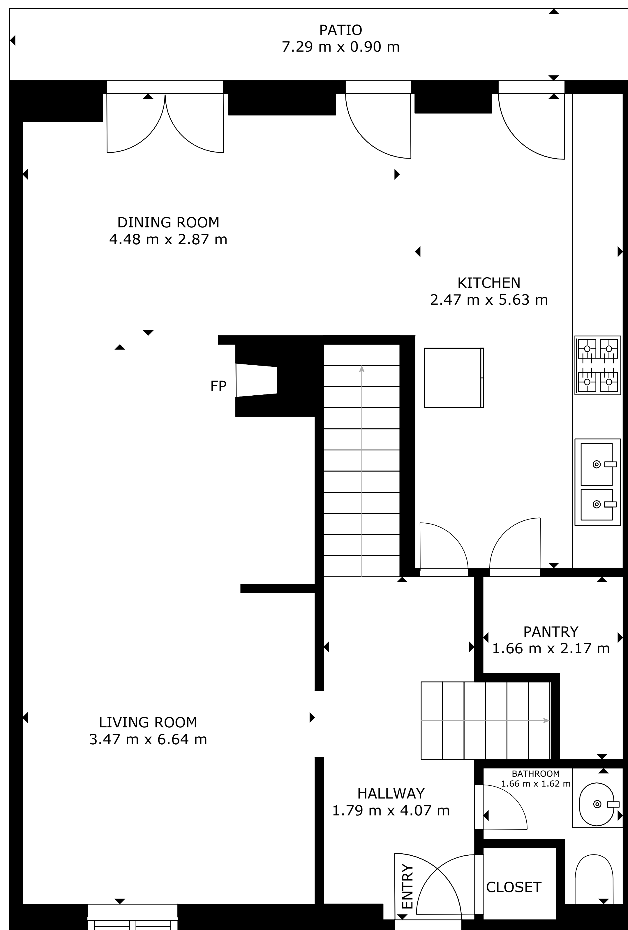
FLOOR 2
