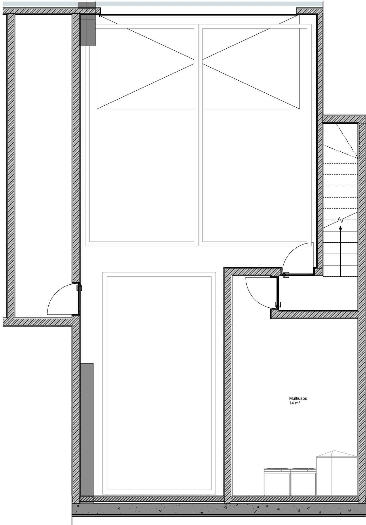
V07_AS.T4.7 - Box 1:50
