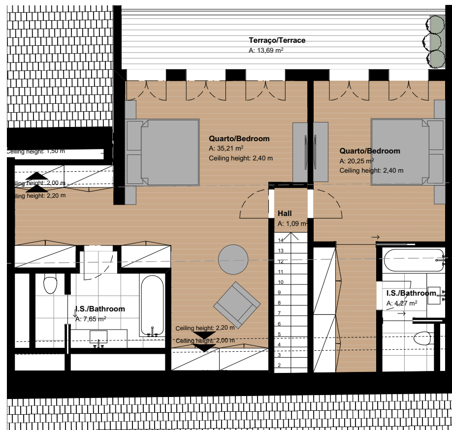
Floor Level 18.75
