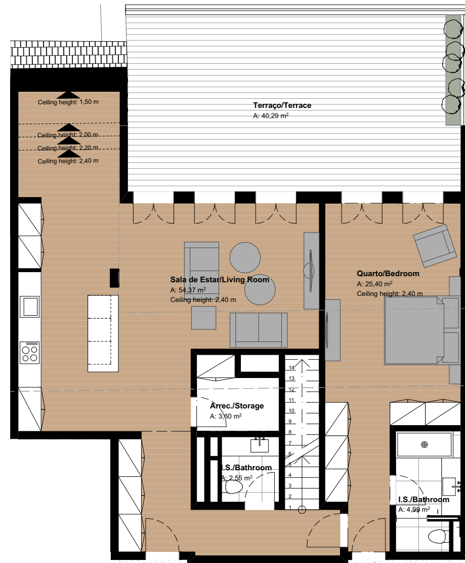
Floor Level 16.10
