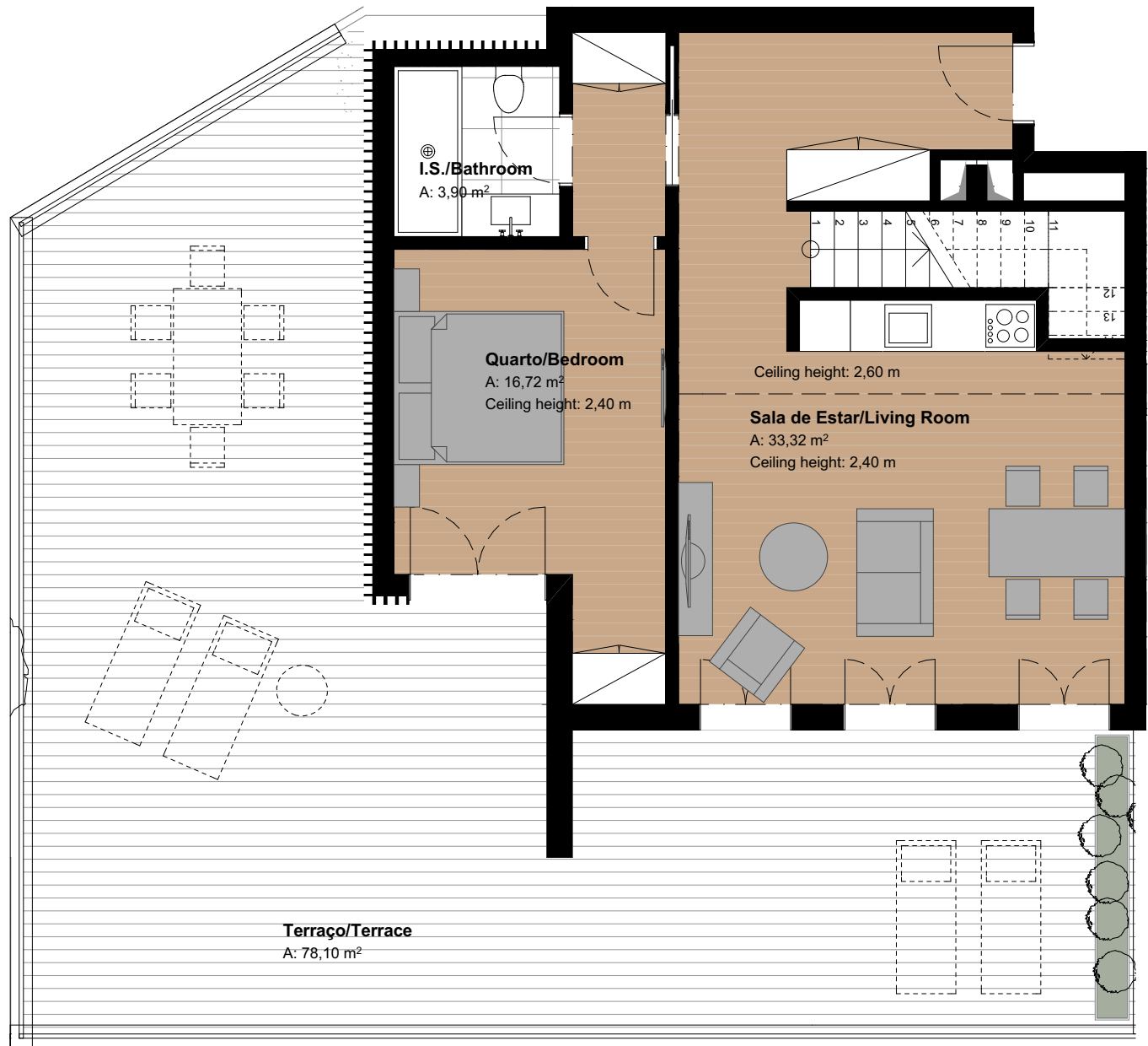
Floor Level 19.65
