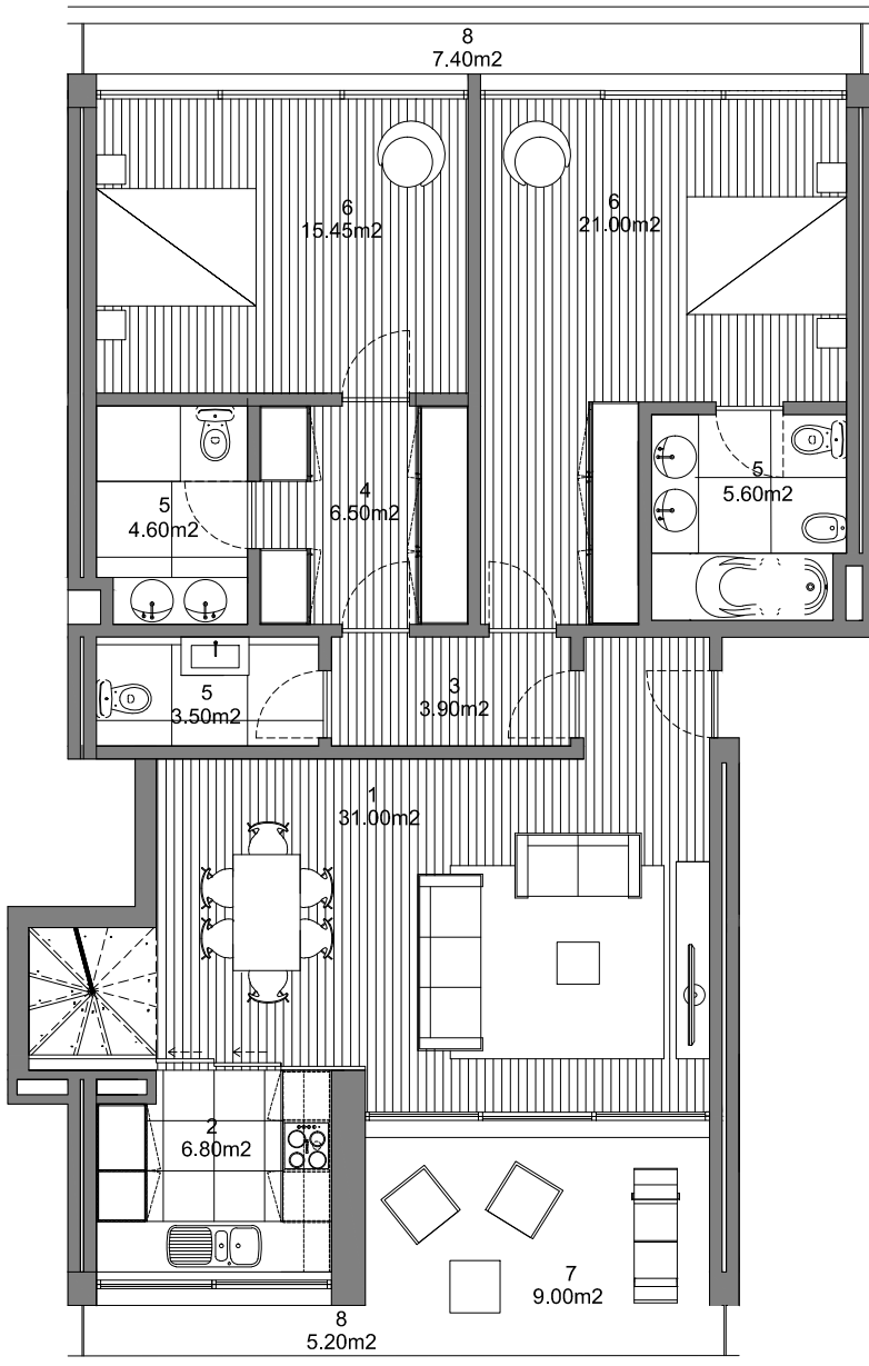
SECOND FLOOR
